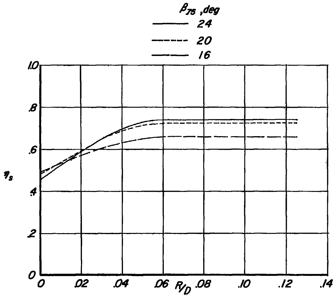
Figure 5.- Effect of lip radius ratio on static thrust efficiency at several blade angles. \frac{l}{D} = 1.03.
