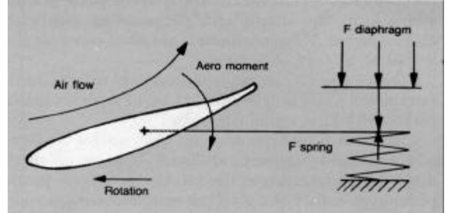
Figure 4 Force Diagram
