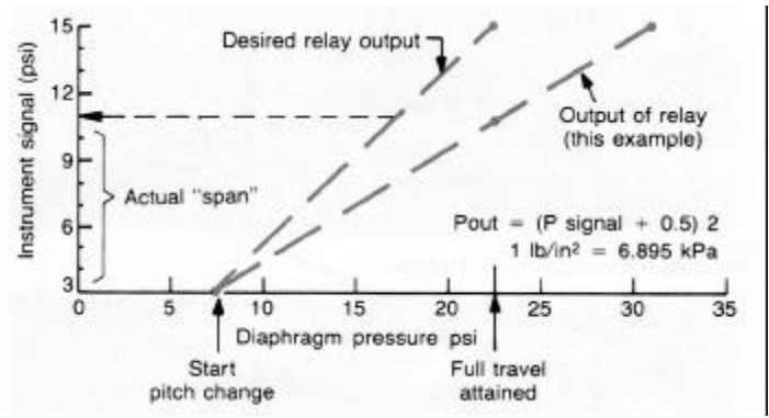
Figure 9 Bias Relay Output
